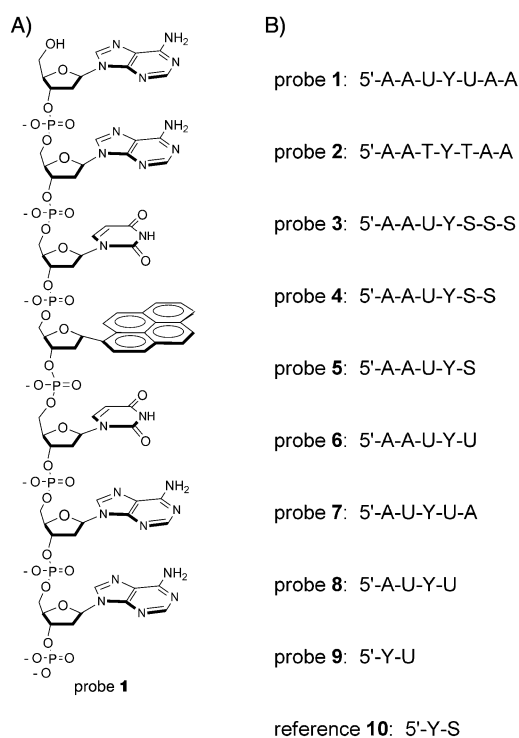
Figure 1. A) Structure of probe 1. B) Sequences of probes in this study. Y = \alpha -pyrene deoxyribose; S = tetrahydrofuran spacer.
